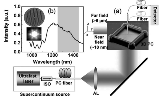
Fig. 1. (a) Setup for supercontinuum generation and coupling into a SNOM. ISO: isolator; AL: achromatic lens. (b) Supercontinuum spectrum. The top inset is a SEM image of the cross section of the PCF. The bottom inset is the mode output of the supercontinuum.
